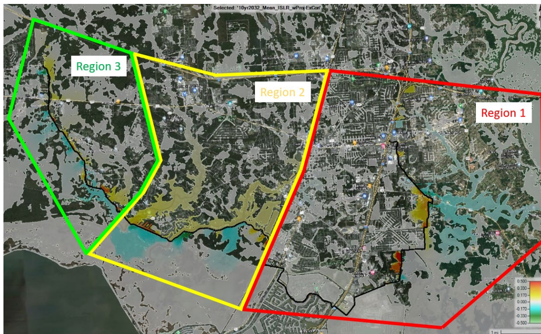
Figure E:14-6. 10-year 2032 event difference map depicting WSE increases and lowering's for the intermediate rate of SLR and mean inflows on the Bogue Chitto River and Pearl River. Regions correlate to areas discussed in the following results section. For a comprehensive description of difference maps refer to Annex 3 of this appendix.
