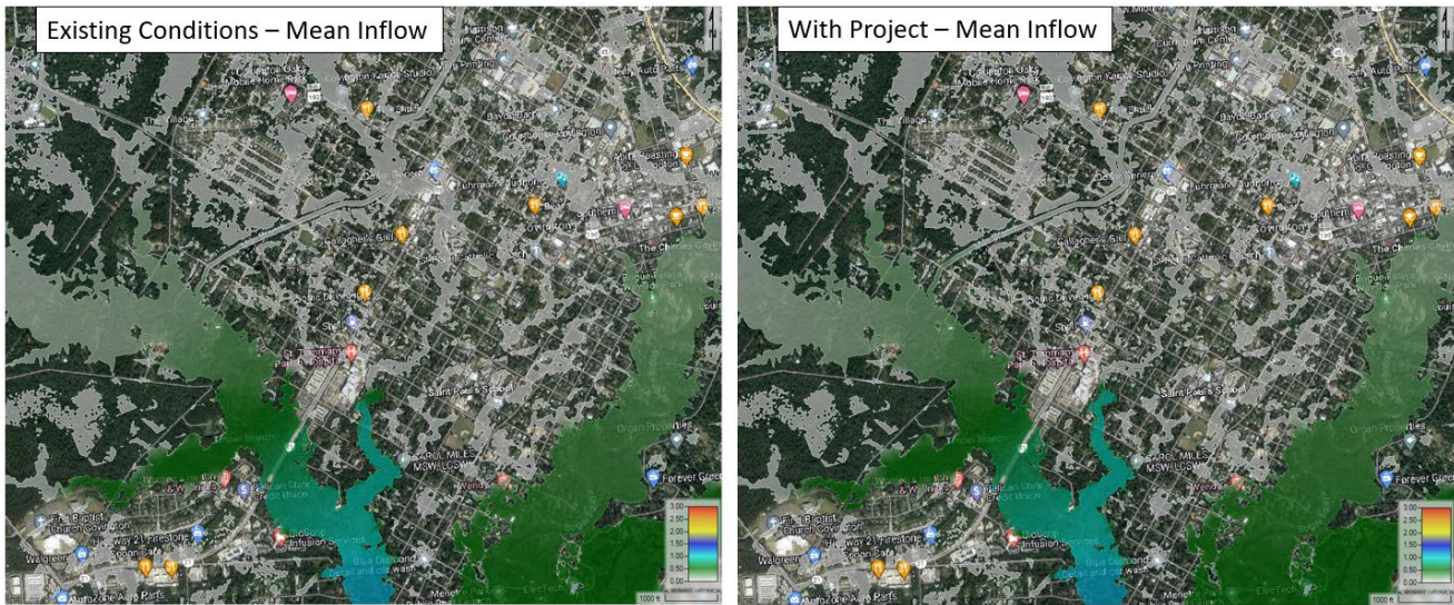
Figure E:14-16. 10-year 2082 event, Existing Condition (left) and With Project (right), depicting the change in WSE between the HSLR-LSLR simulations with mean inflows on the Pearl River and Bogue Chitto River; zoomed into Mile Branch project area
