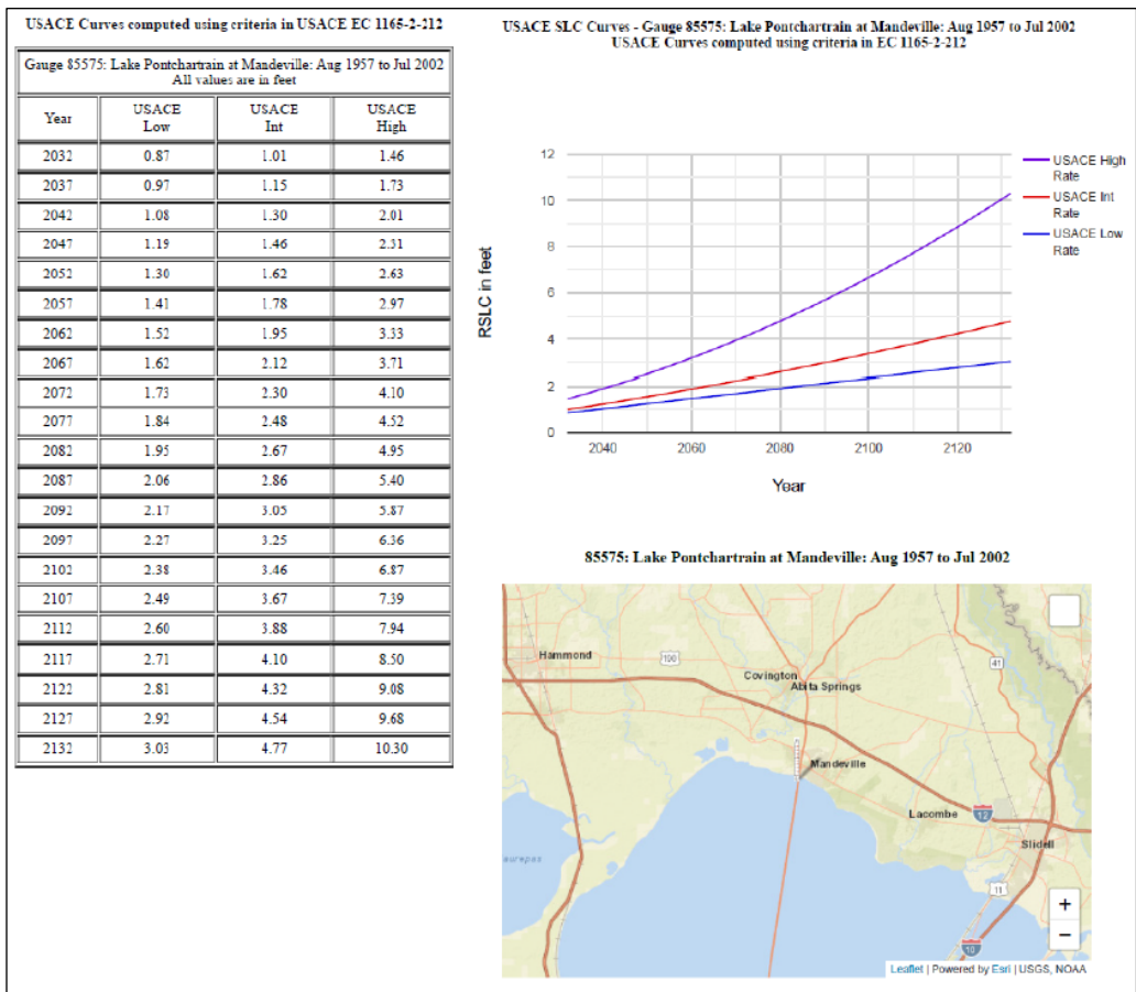
Figure E:3-3. USACE Sea Level Change Curves
