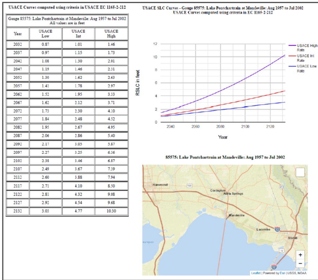
Figure E:11-5. USACE Sea Level Change Curves for Mandeville, Louisiana
