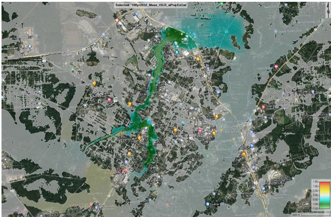
Figure E3:45. 100-year 2032 ISLR difference in WSE with project
