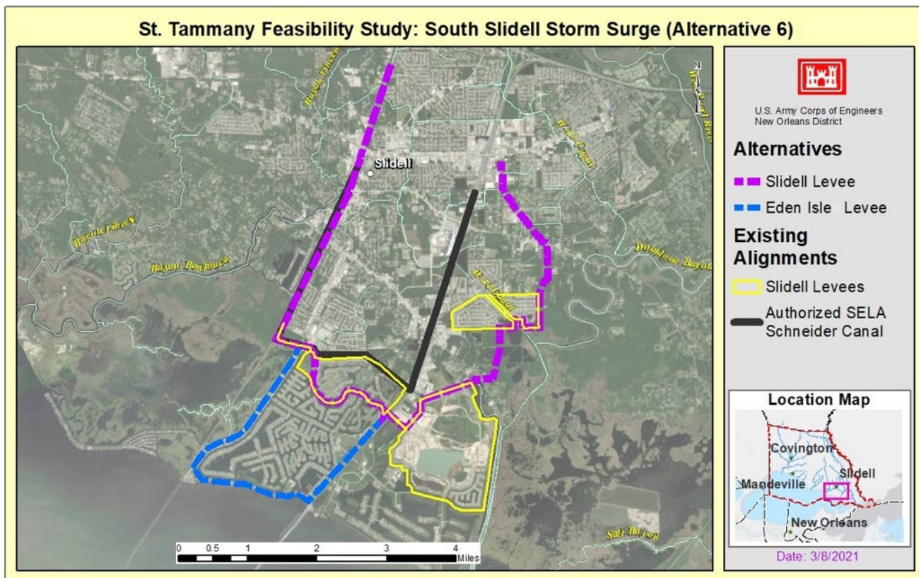
Figure E:6-14. Alternative 6 Measures: Proposed Slidell Levee Alignment and Eden Isle Levee
