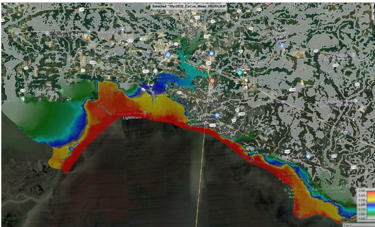
Figure E3:73. 10-year 2032 existing condition HSLR minus LSLR
