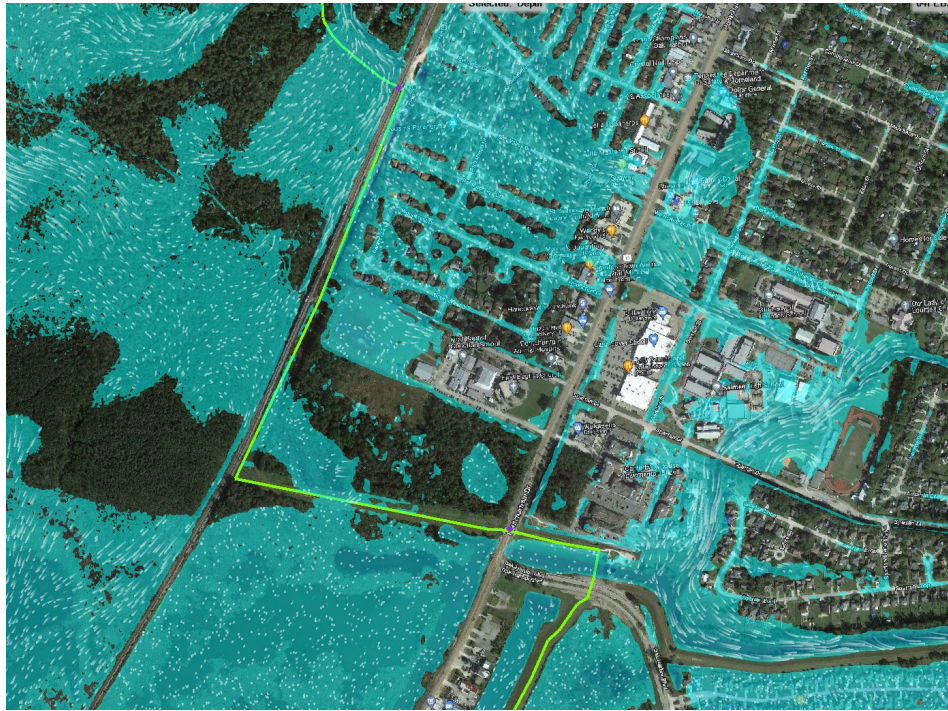
Figure E5:23. Segment 8 Existing Conditions
