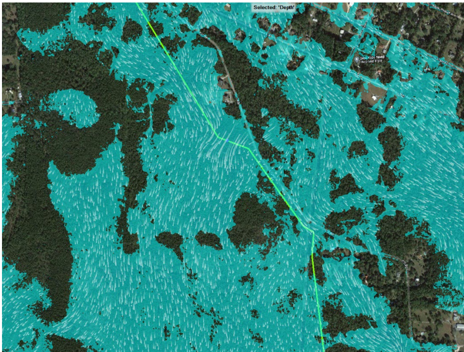
Figure E5:9. Segment 3 With Project
