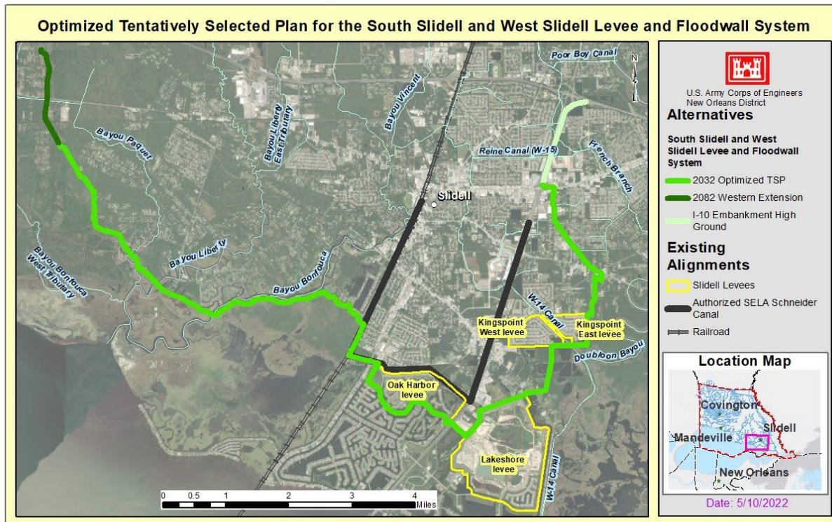
Figure E:14-5. RP for the South Slidell and West Slidell Levee and Floodwall System
