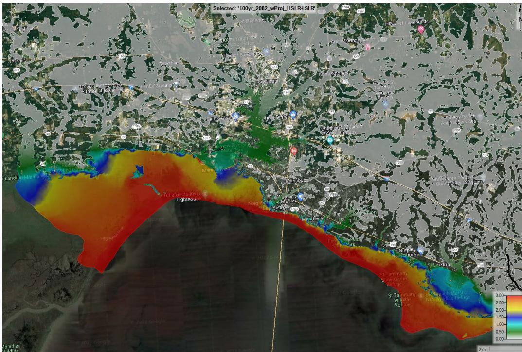
Figure E3:64. 100-year 2082 with-project HSLR minus LSLR
