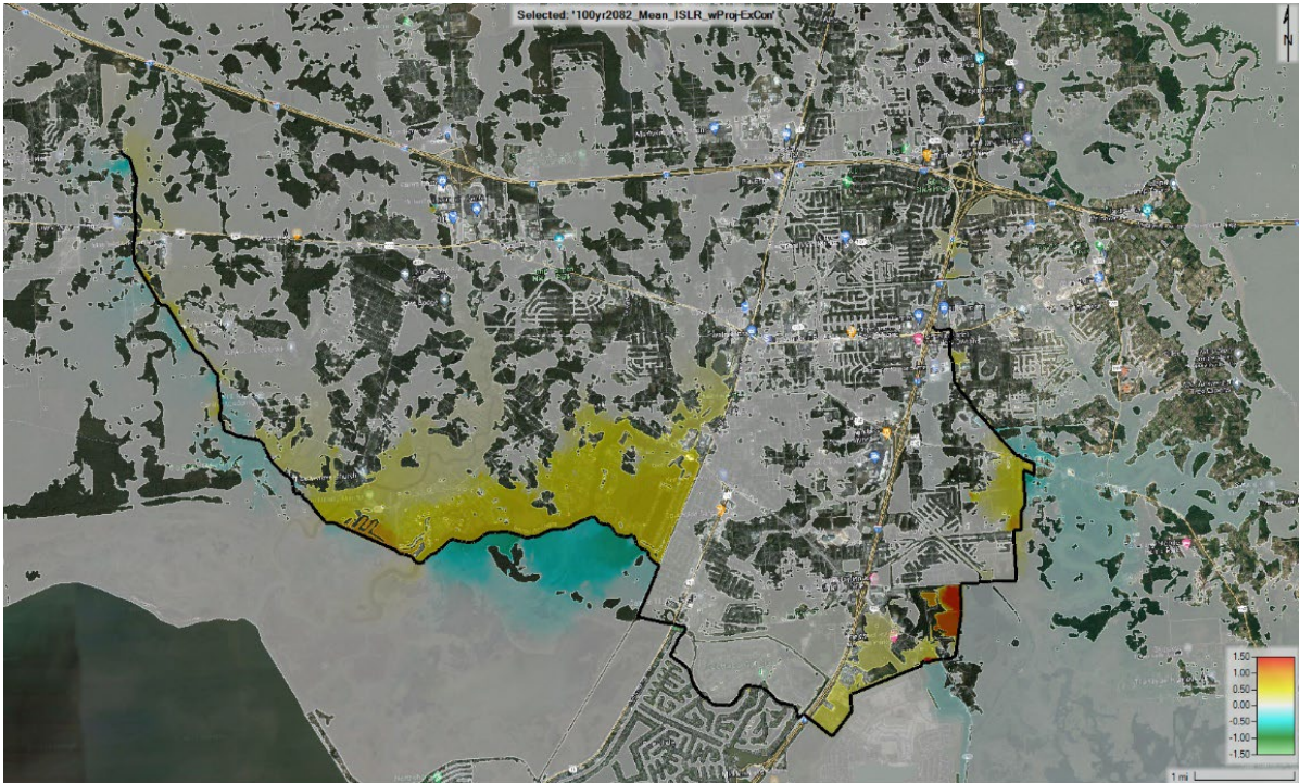
Figure E3:34. 100-year 2082 ISLR difference in WSE with project
