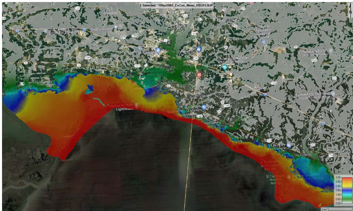
Figure E3:76. 100-year 2082 existing condition HSLR minus LSLR
