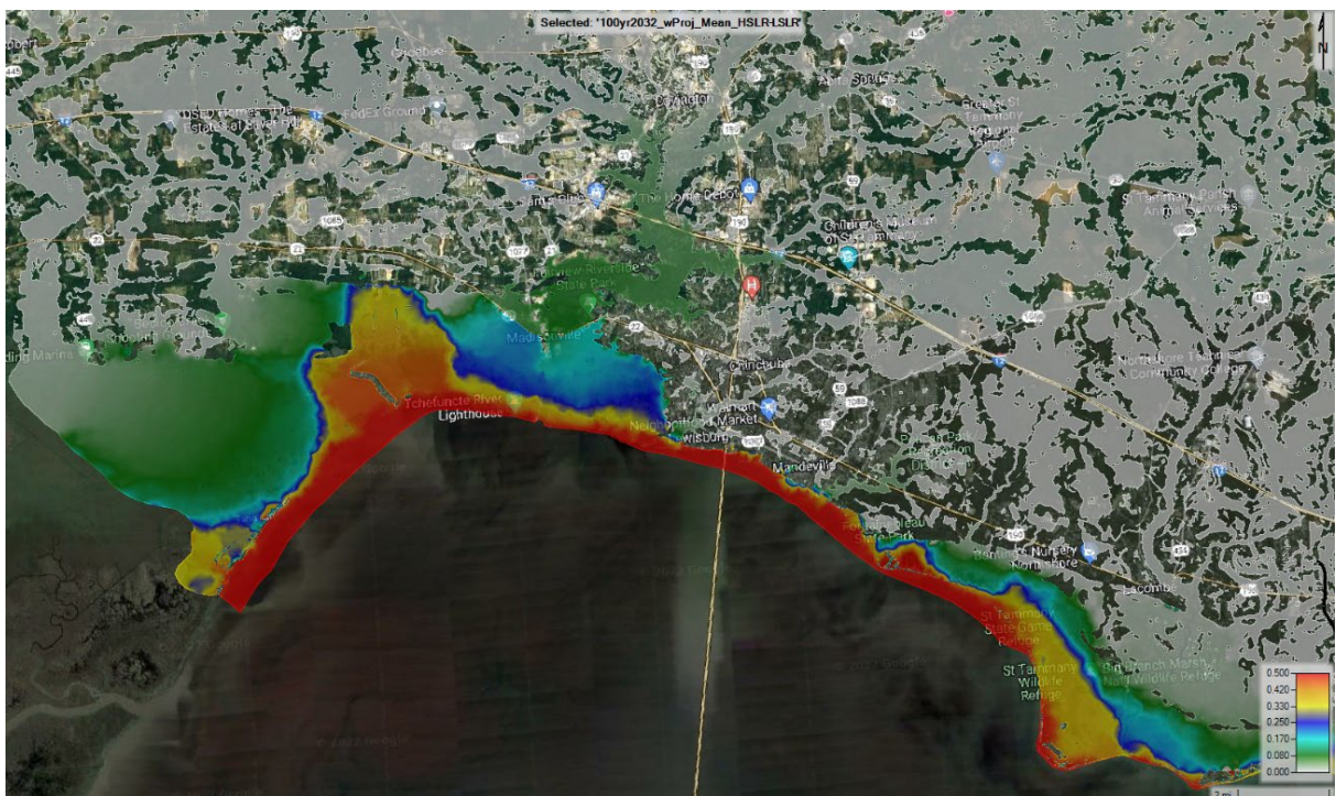
Figure E3:79. 100-year 2032 with-project HSLR minus LSLR
