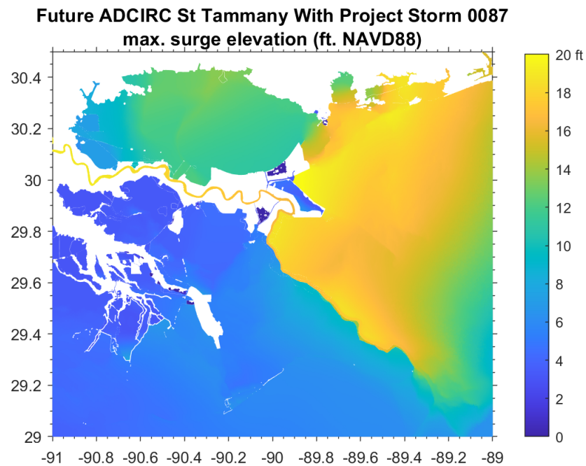
Figure E:13-5. Sample plot of WSE for a future-year with-project simulations from a specific synthetic storm.
