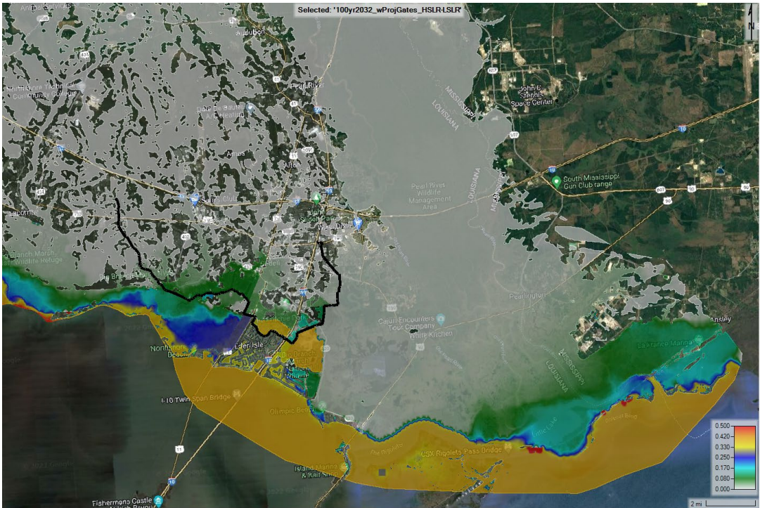
Figure E3:55. 100-year 2032 with-project HSLR minus LSLR
