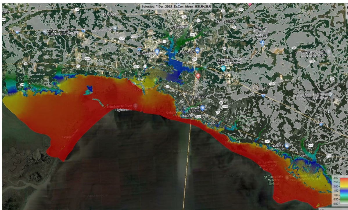
Figure E3:74. 10-year 2082 existing condition HSLR minus LSLR
