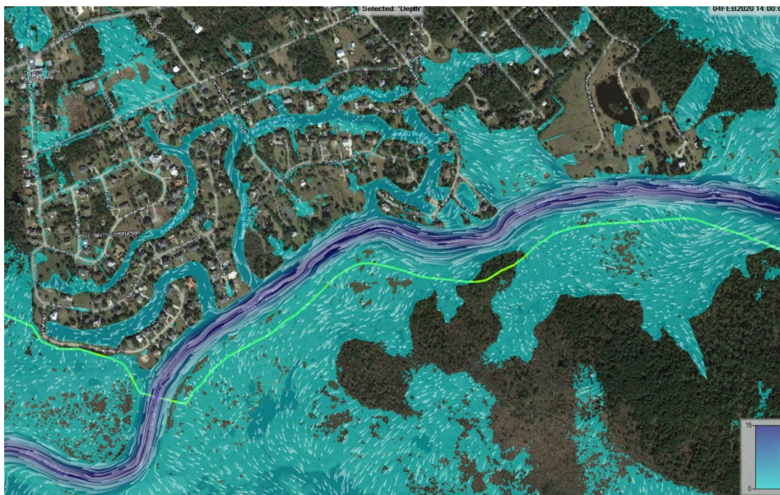
Figure E5:17. Segment 6 Existing Conditions
