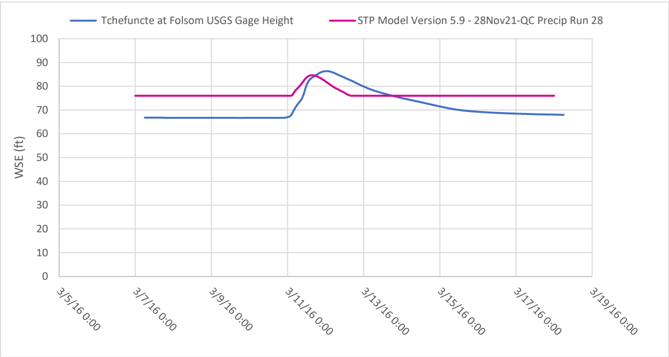
Figure E4:9. March 2016 calibration event plot for USGS Gage -Tchefuncte River at Folsom, LA
