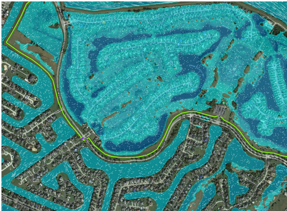
Figure E5:27. Segment 9 With Project
