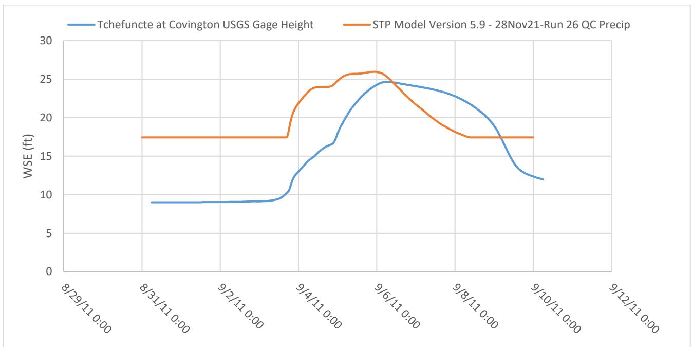
Figure E4.3. September 2011 calibration event plot for USGS Gage -Tchefuncte River at Covington, LA
