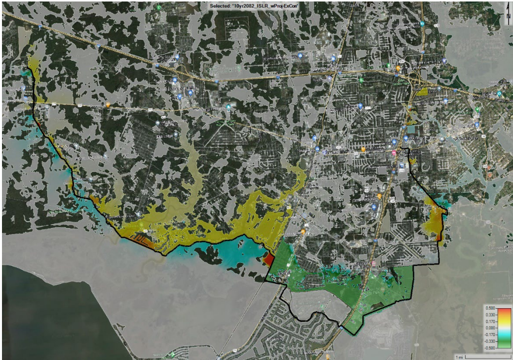
Figure E3:4. 10-year 2082 ISLR difference in WSE with project
