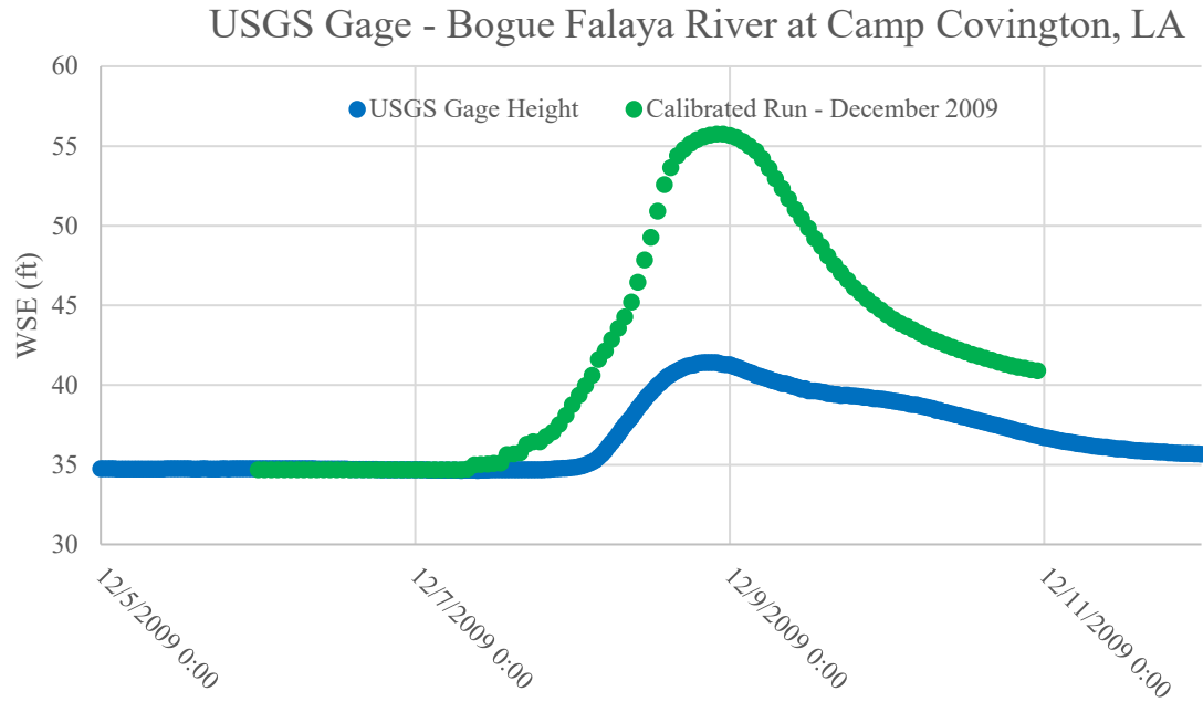
Figure E2:17. December 2009 calibration event plot for USGS Gage -Bogue Falaya River at Camp Covington, LA
