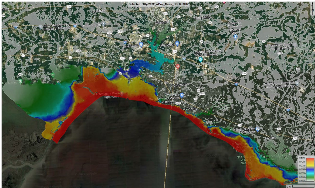
Figure E3:77. 10-year 2032 with-project HSLR minus LSLR
