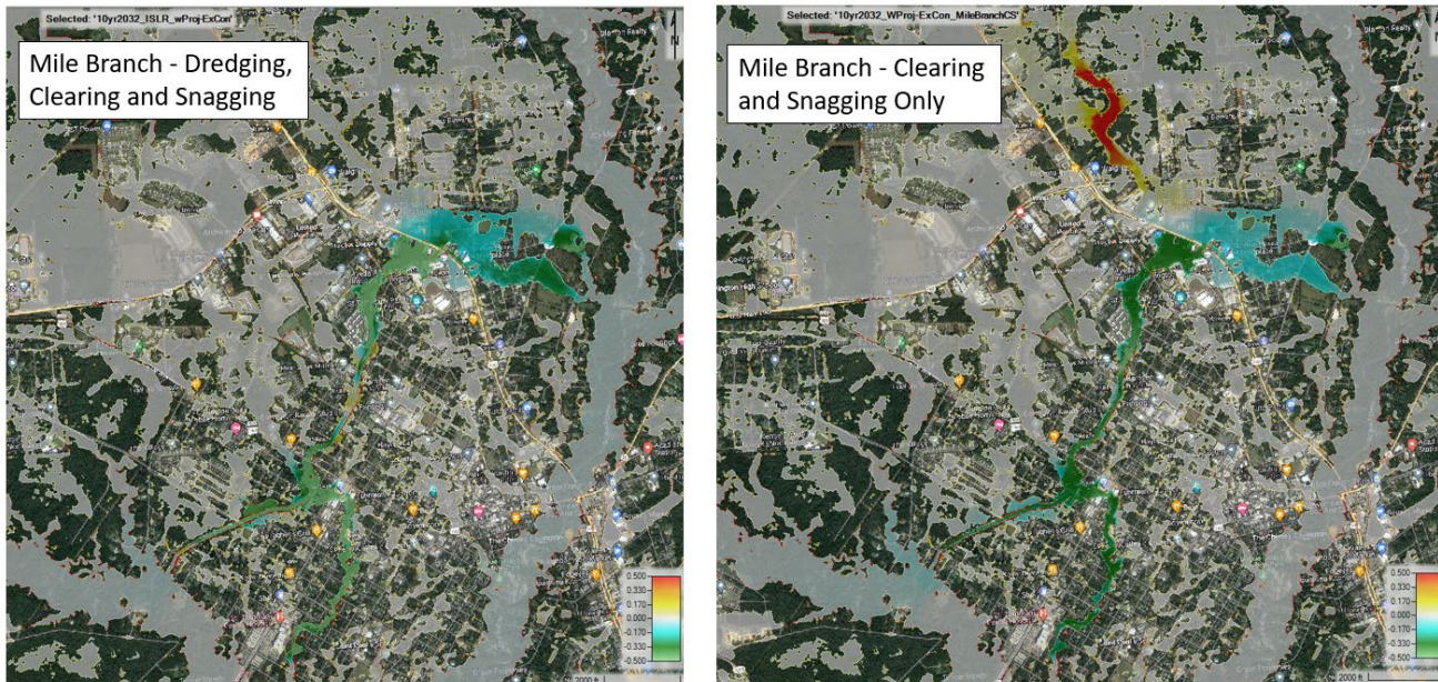
Figure E:14-3. Difference maps for the 10-year 2032 event with the intermediate sea level rise (ISLR) rate at Lake Pontchartrain, in the vicinity of Mile Branch comparing the Optimized _____ TSP with dredging, clearing and snagging of the channel (left) and only clearing and snagging of the channel (right).
