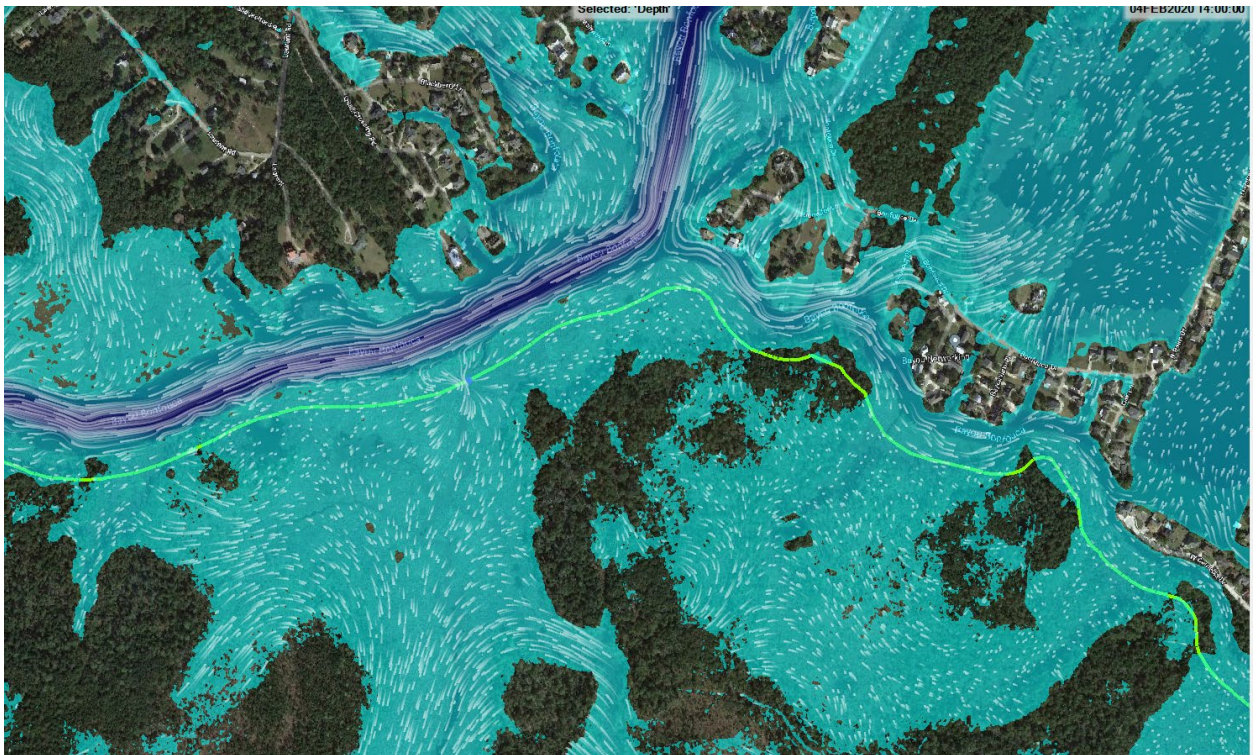
Figure E5:21. Segment 7 With Project
