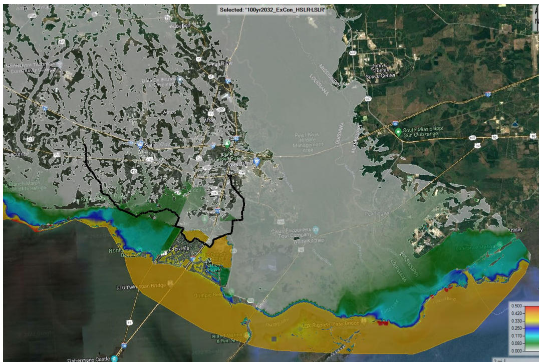
Figure E3:51. 100-year 2032 existing condition HSLR minus LSLR
