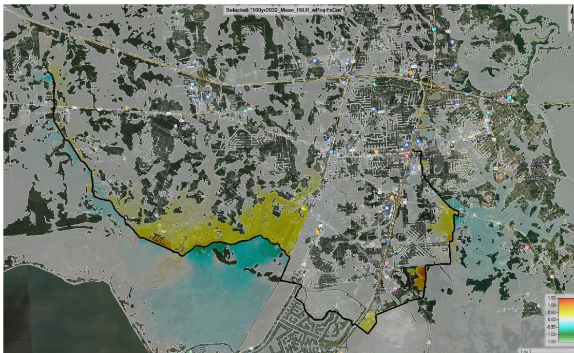
Figure E3:33. 100-year 2032 ISLR difference in WSE with project
