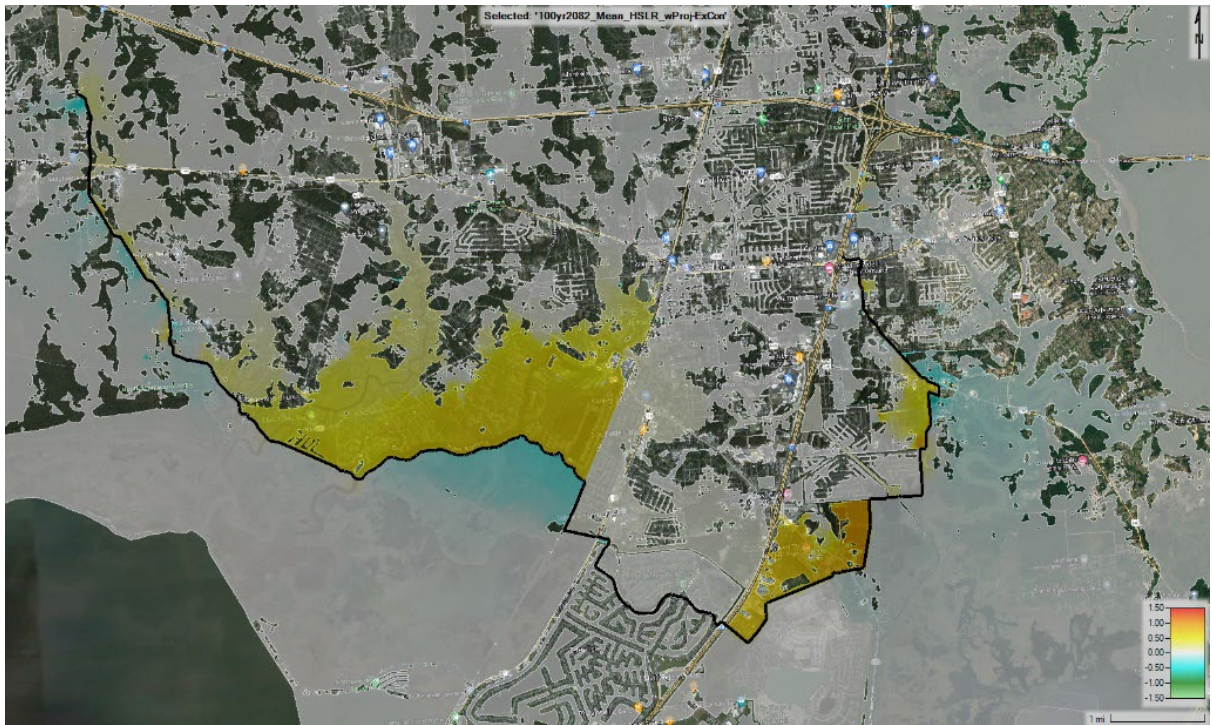
Figure E3:36. 100-yr 2082 HSLR difference in WSE with project
