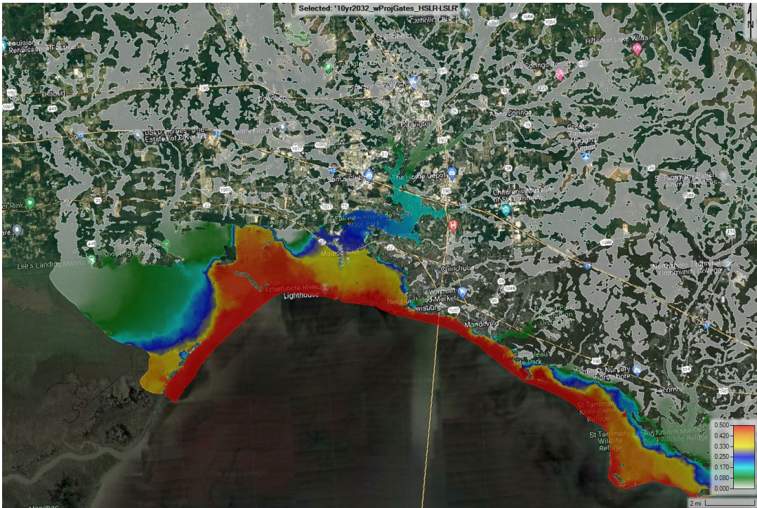
Figure E3:61. 10-year 2032 with-project HSLR minus LSLR
