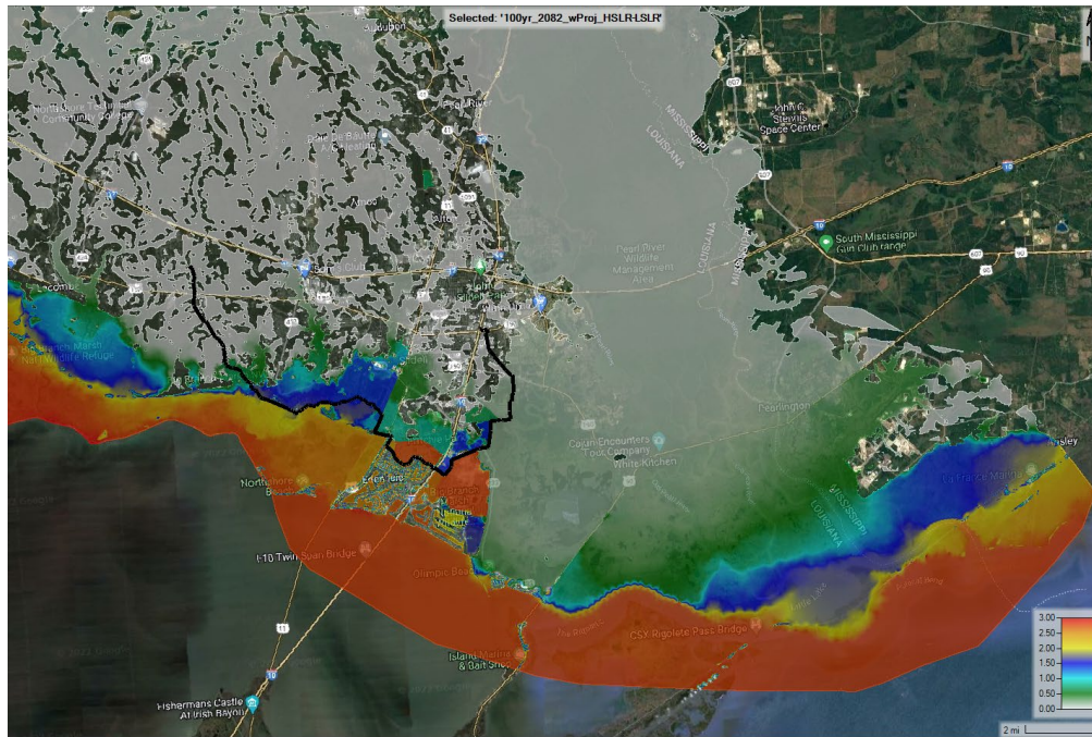
Figure E:14-13. 100-year 2082 event with-project HSLR-LSLR with frequency inflows on the Pearl River and Bogue Chitto River
