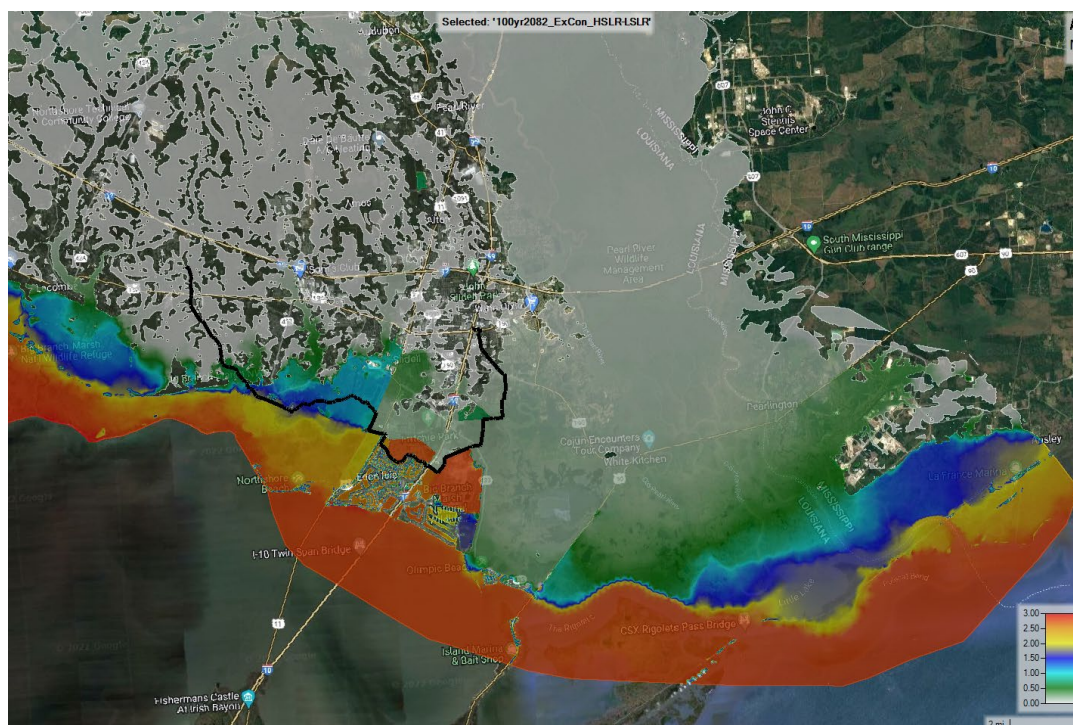
Figure E3:52. 100-year 2082 existing condition HSLR minus LSLR
