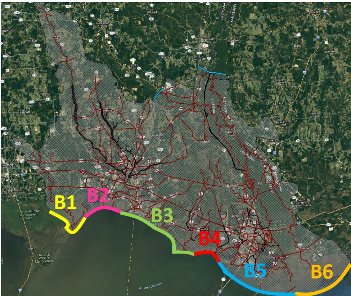
Figure E:12-4. Locations of Downstream Boundary Conditions B1-B6
