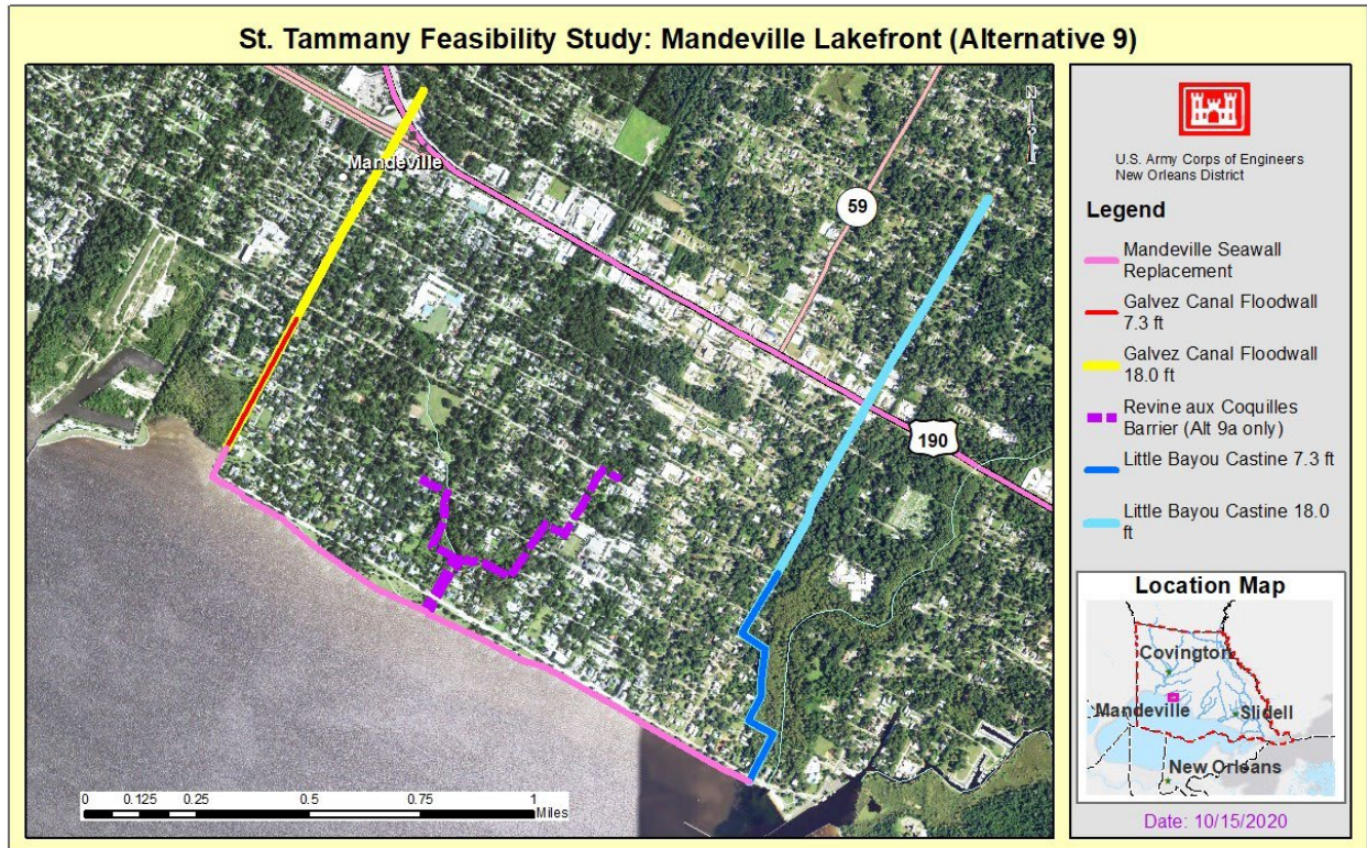
Figure E:6-17. Alternative 9 Measures: Mandeville Seawall Replacement, Galvez Canal Floodwall, Ravine Aux Coquilles Passive Barrier, and Little Bayou Castine Passive Barrier
