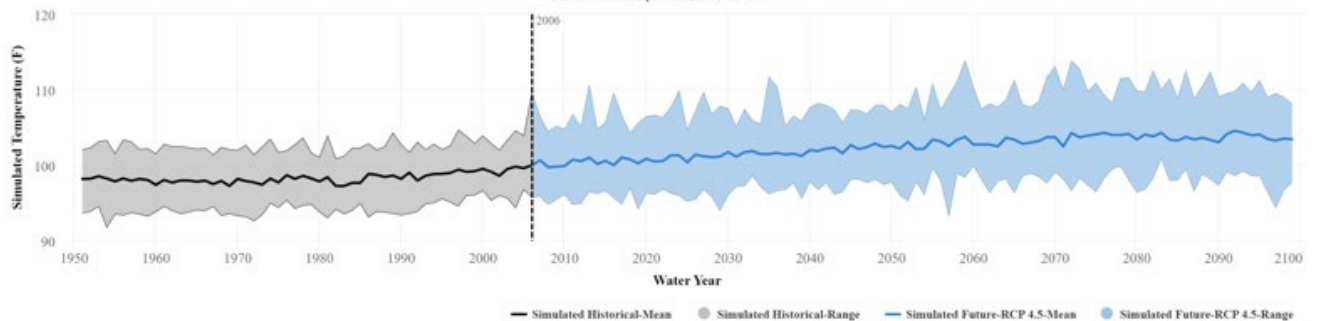
Figure E:11-9. South Atlantic-Gulf Region 03 CHAT results depicting annual-maximum of mean streamflow, annual-maximum 1-day precipitation, and annual-maximum temperature for the Pearl HUC-4 Basin, Lower Pearl HUC-8 Basin
