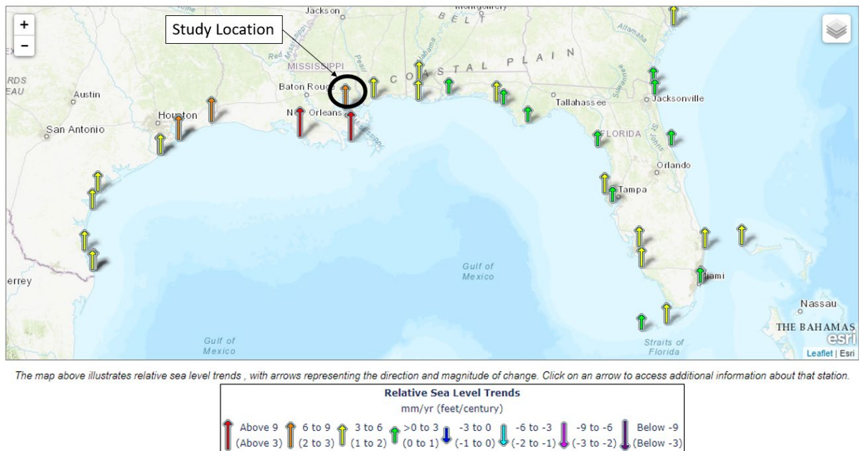
Figure E:11-1. Sea level trends measured by tide gages presented as local RSL trends as opposed to global sea level trend. 1
