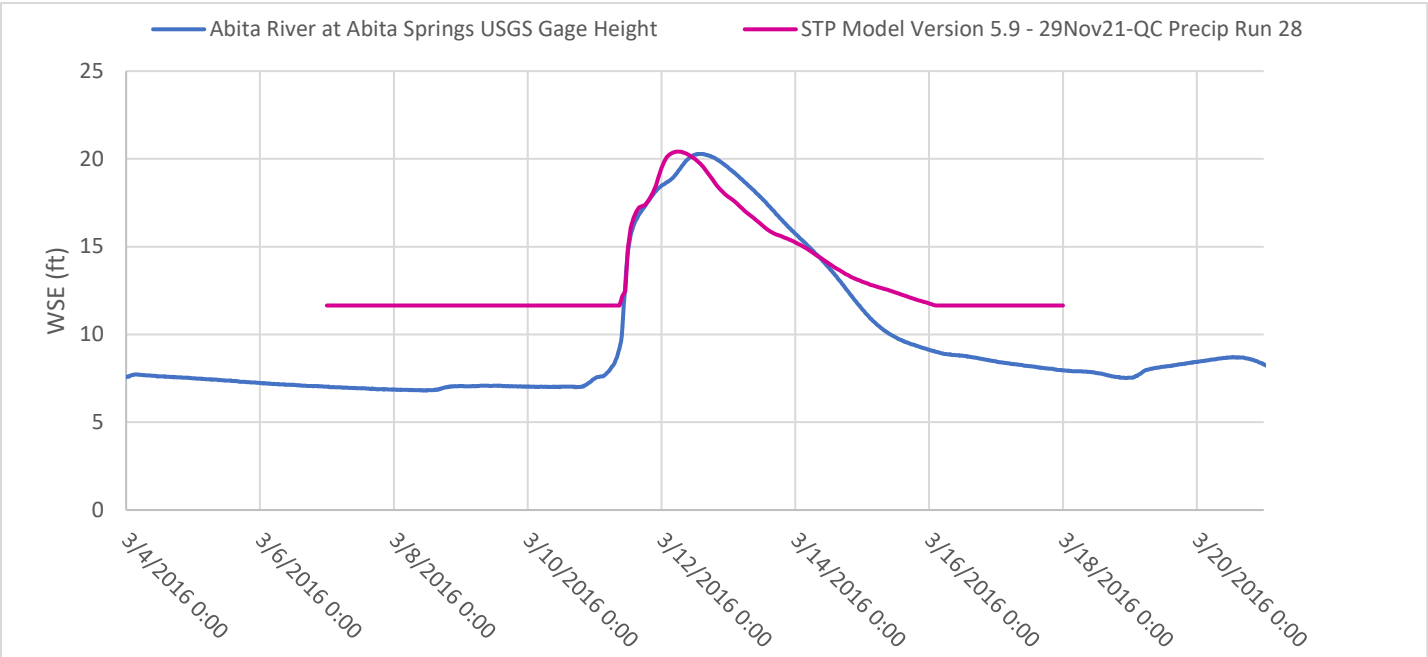
Figure E4:14. March 2016 calibration event plot for USGS Gage – Abita River at Abita Springs, LA
